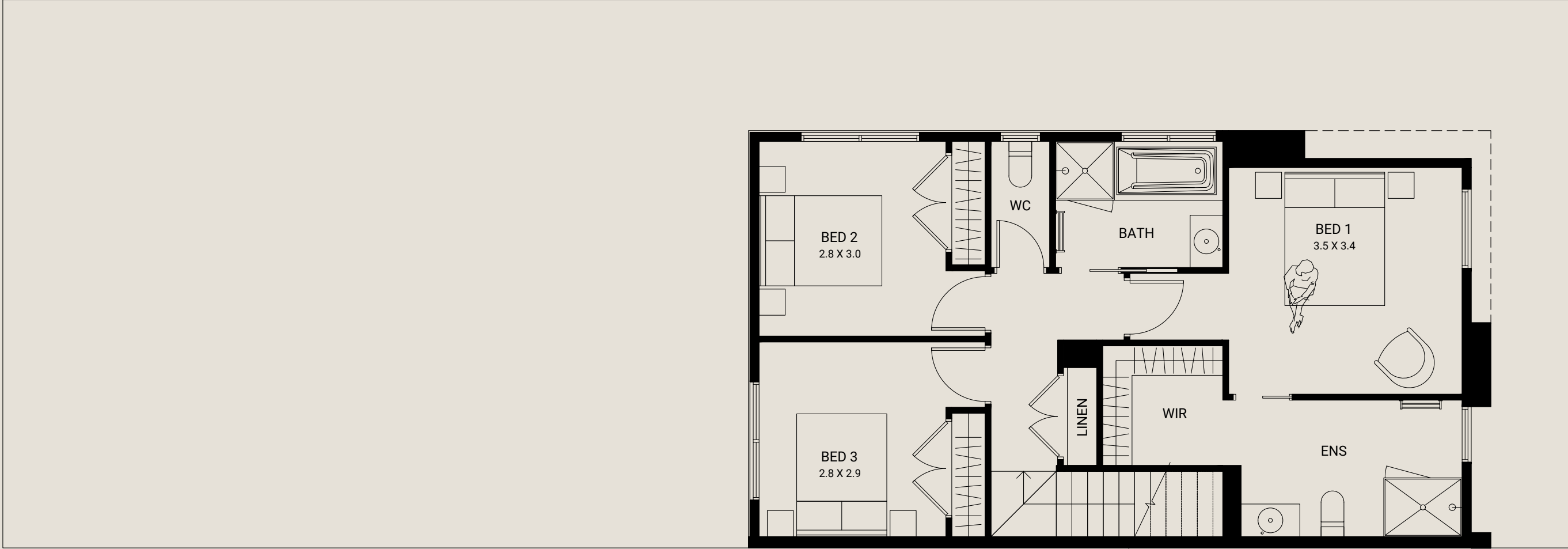
FIRST FLOOR
