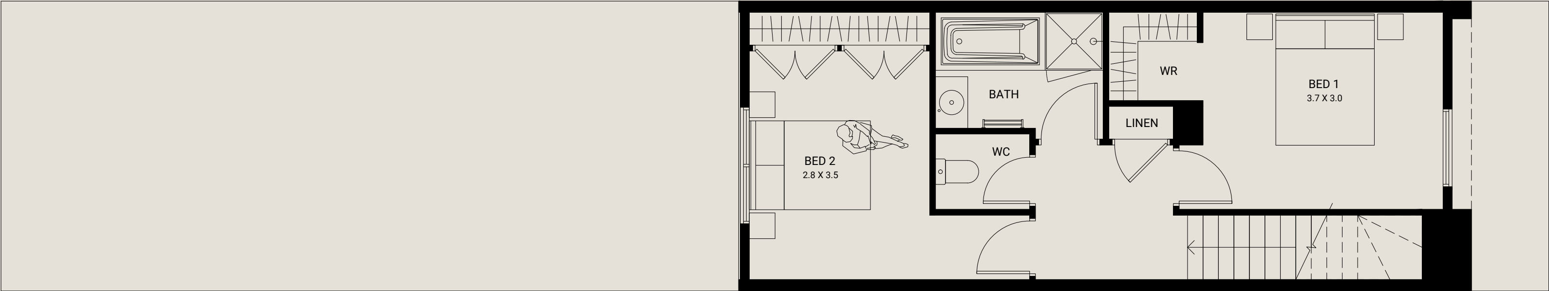
FIRST FLOOR
