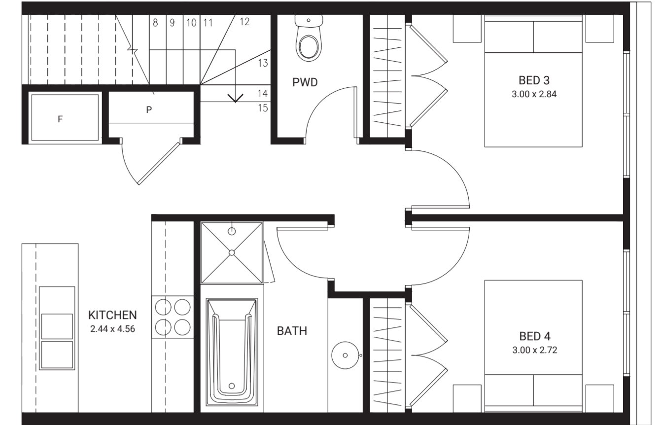
FIRST FLOOR SEPARATE WC OPTION
