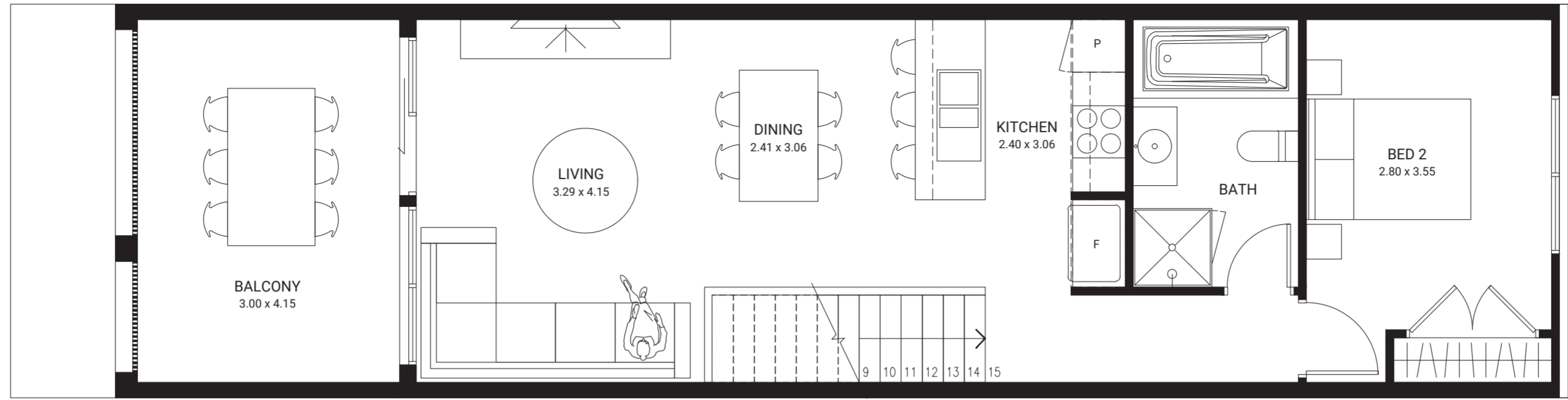
FIRST FLOOR
