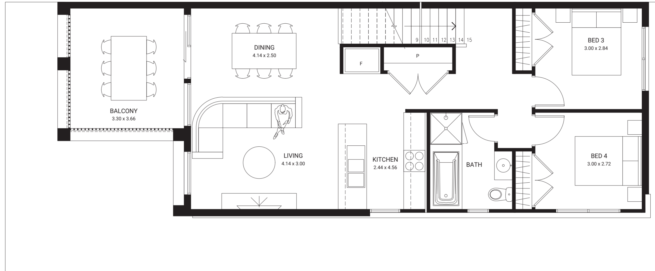
FIRST FLOOR
